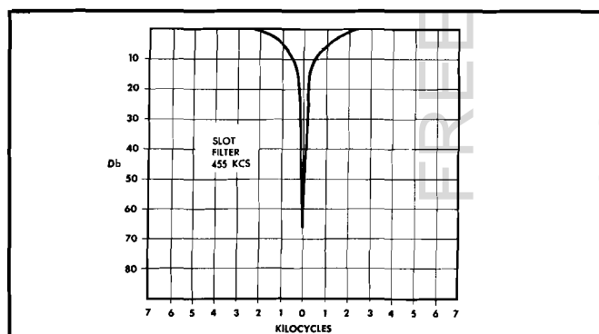
Figure 7. Slot Filter Response Curve
