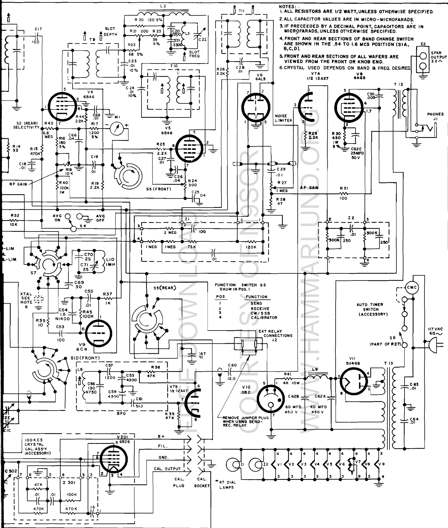
Figure 12. Hammarlund HQ-145X Communications Receiver, Schematic Diagram
