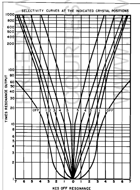
Figure 6. Selectivity Curves
