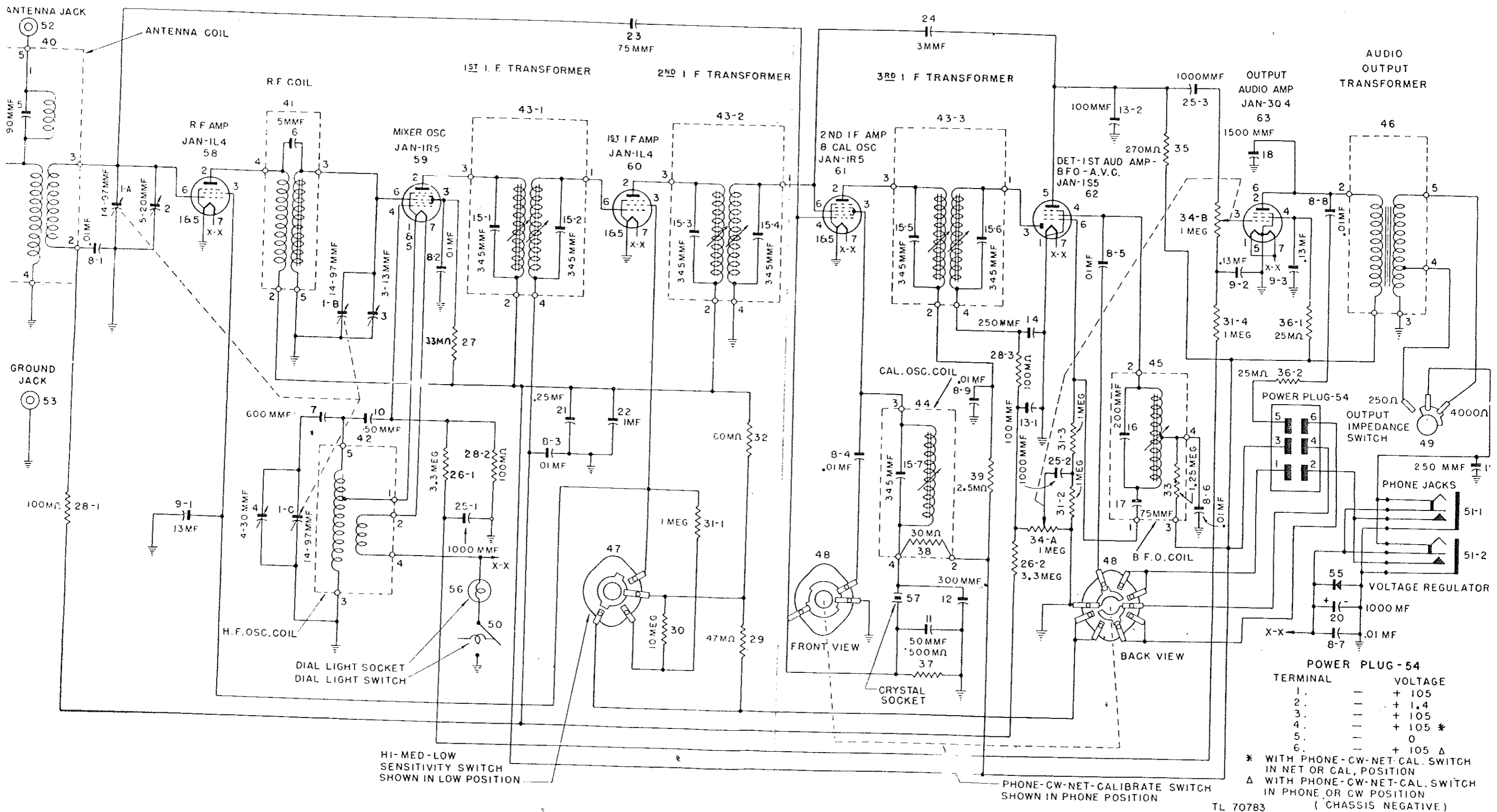
Figure 57. Receiver schematic diagram of Radio Receiver and Transmitter BC-1307.
