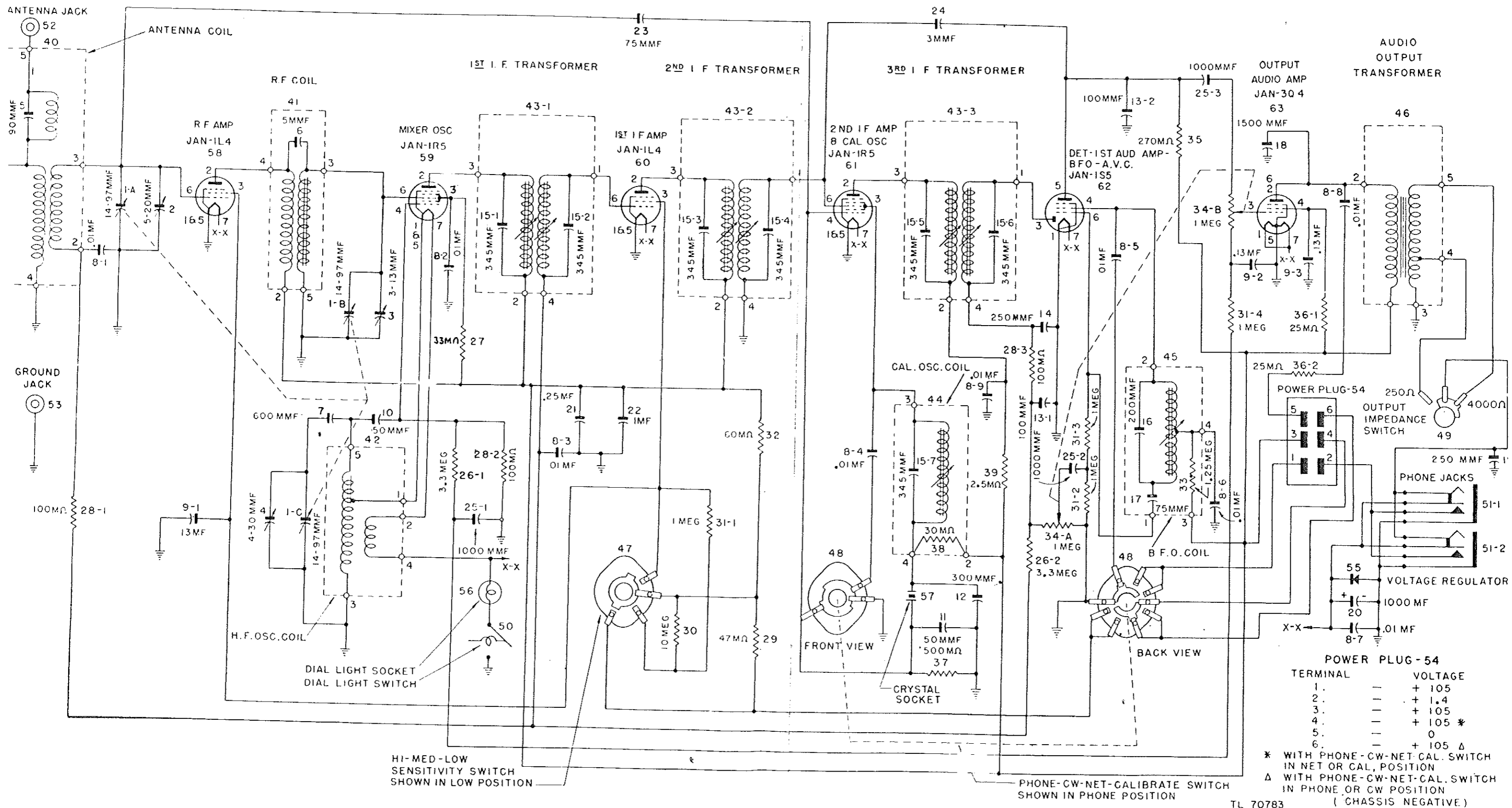
Figure 57. Receiver schematic diagram of Radio Receiver and Transmitter BC-130.
